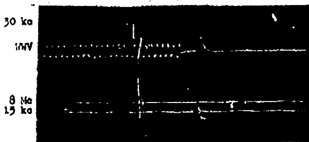
Fig. 3.83 Narrow-band responses Shot No. 8 1000 km from ground zero
